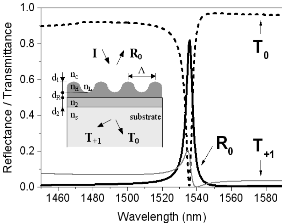
Fig. 11. Calculated spectral filter response with parameters corresponding to those of the fabricated filter for TE polarization. The parameters are as follows: thicknesses, d_1 = 333 nm, d_R = 0 nm (No residue), d_2 = 250 nm; refractive indices n_H = 1.51 , n_L = 1.00 , n_2 = 1.87 , n_c = 1.00 , n_s = 1.50 ; grating period \Lambda = 1111 nm; incident angle \theta_{in} = 10^\circ
